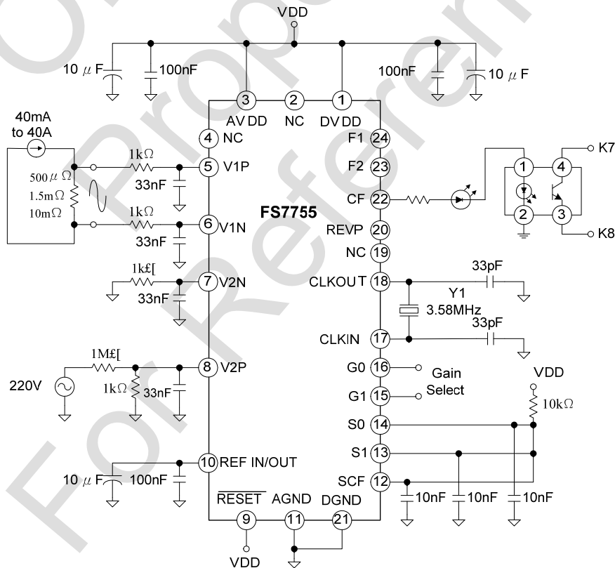
Fig3 Application Circuit
