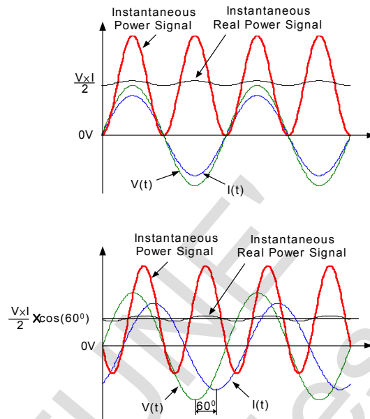
Fig6 DC Component of Instantaneous Power Signal Conveys Real Power Information (PF ≤ 1)
