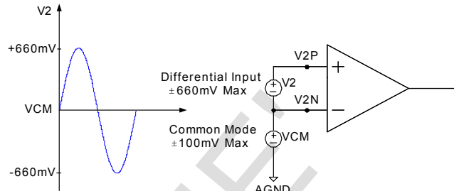
Fig8 Maximum Signal Levels (Channel 2)
