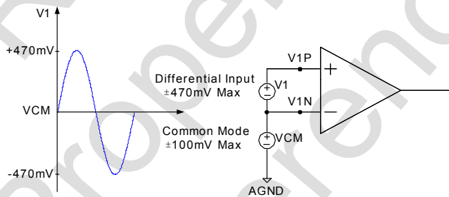
Fig7 Maximum Signal Levels (Channel 1, Gain = 1)
