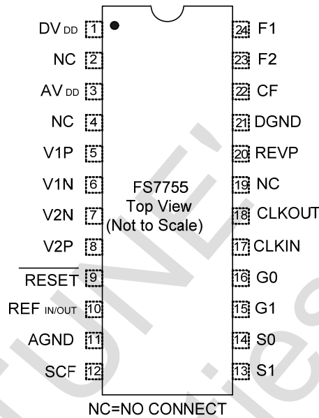
Fig1 Pin Configuration
