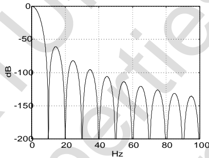
The Frequency Response Diagram of FS511 Digital Filter
