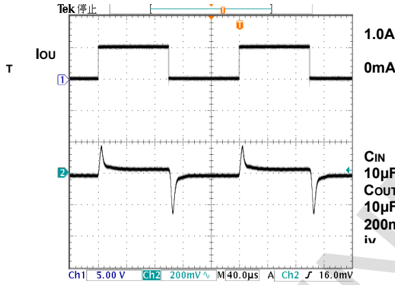
Load Transient
