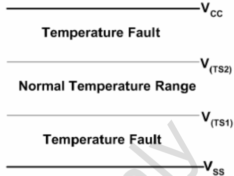
Figure 4. TS Input Thresholds
