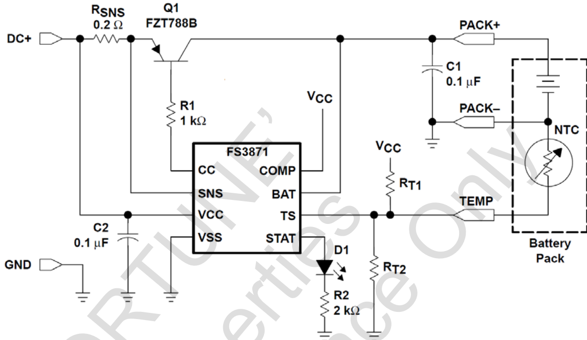
Figure 1. FS3871 Typical Application for one cell
